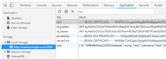
Fig. 4. Local storage information after successful login
